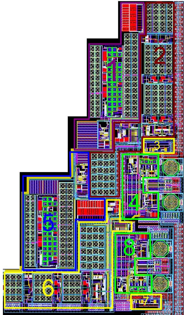
Figure 2: Intermediate frequency amplifier layout
