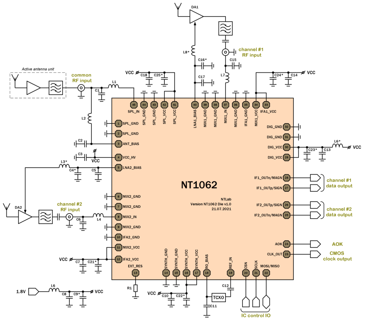
Figure 4.7: NT1062 bare die application schematic
