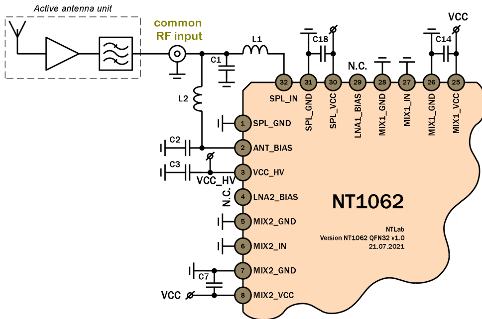
Figure 4.4: NT1062 QFN32 specific application schematic (common RF input)
