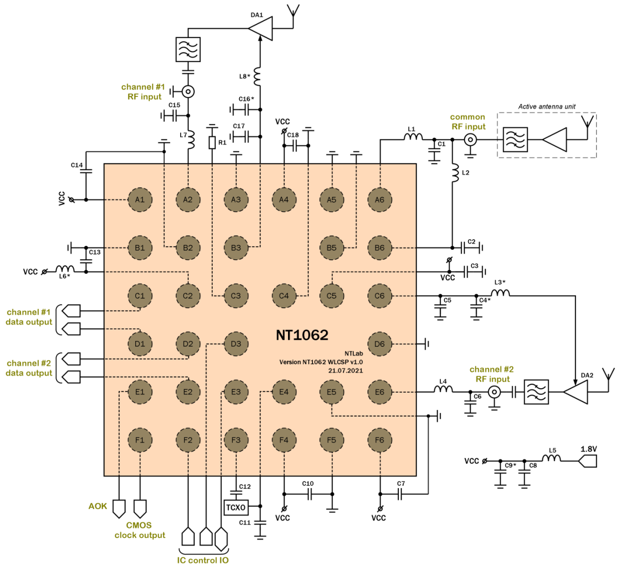
Figure 4.6: NT1062 WLCSP (top view) application schematic
