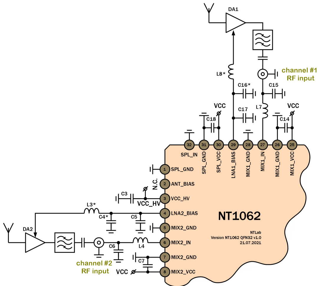
Figure 4.5: NT1062 QFN32 specific application schematic (separate RF inputs)
